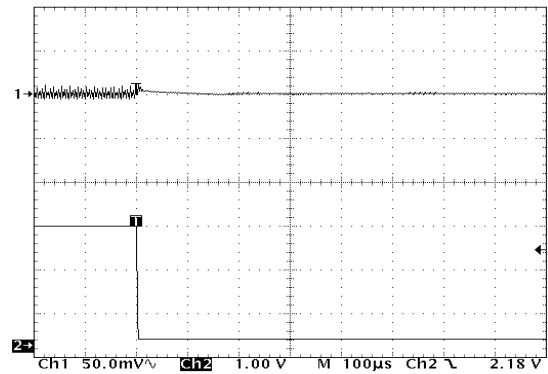
Figure 35. NCP1400ASN19T1 Load Transient Response
