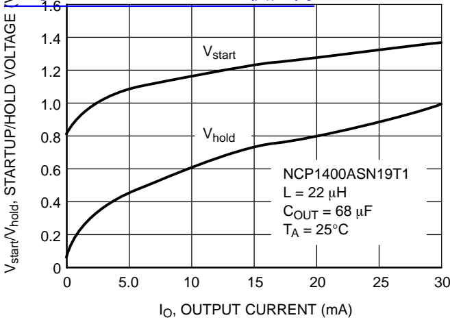
Figure 26. NCP1400ASN19T1 Operation Startup/hold Voltage vs. Output Current
