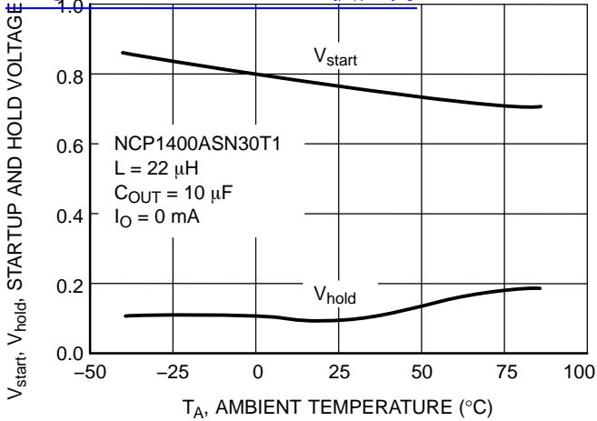
Figure 20. NCP1400ASN30T1 Startup/Hold Voltage vs. Temperature
