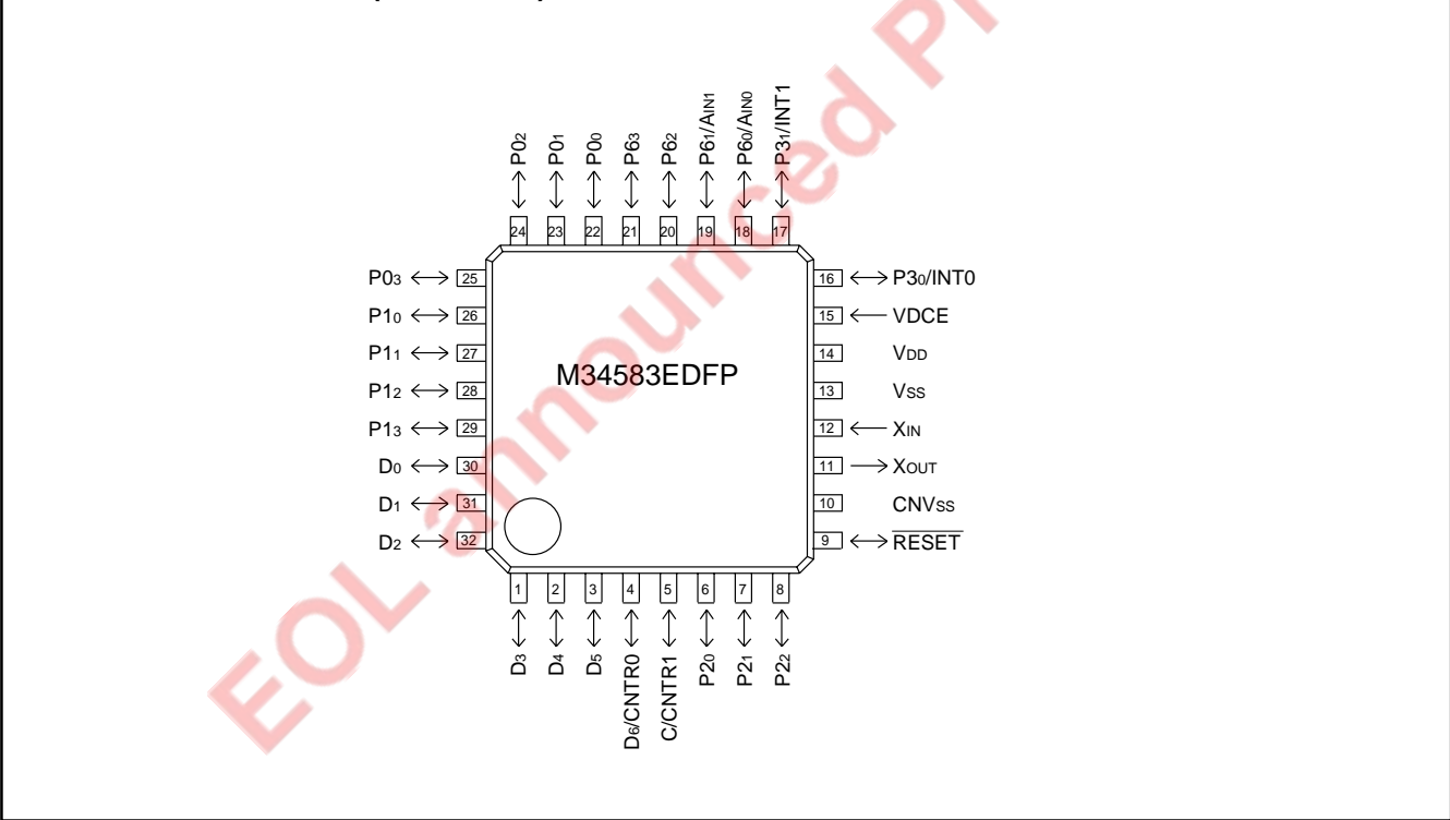
Fig. 69 Pin configuration of built-in PROM version
