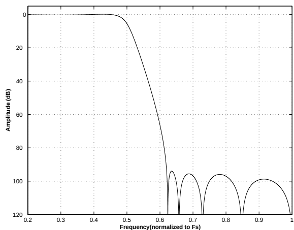
Figure 62. Quad-Speed (fast) Stopband Rejection
