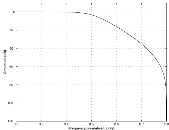
Figure 59. Double-Speed (slow) Transition Band
