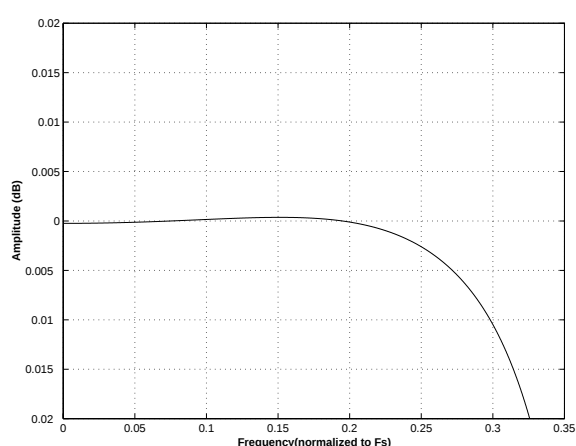
Figure 61. Double-Speed (slow) Passband Ripple
