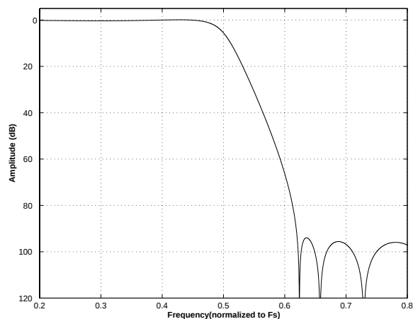
Figure 63. Quad-Speed (fast) Transition Band
