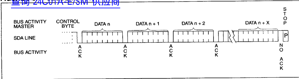
FIGURE 9-3: SEQUENTIAL READ 查询 24C01A E/S/M 供应商
