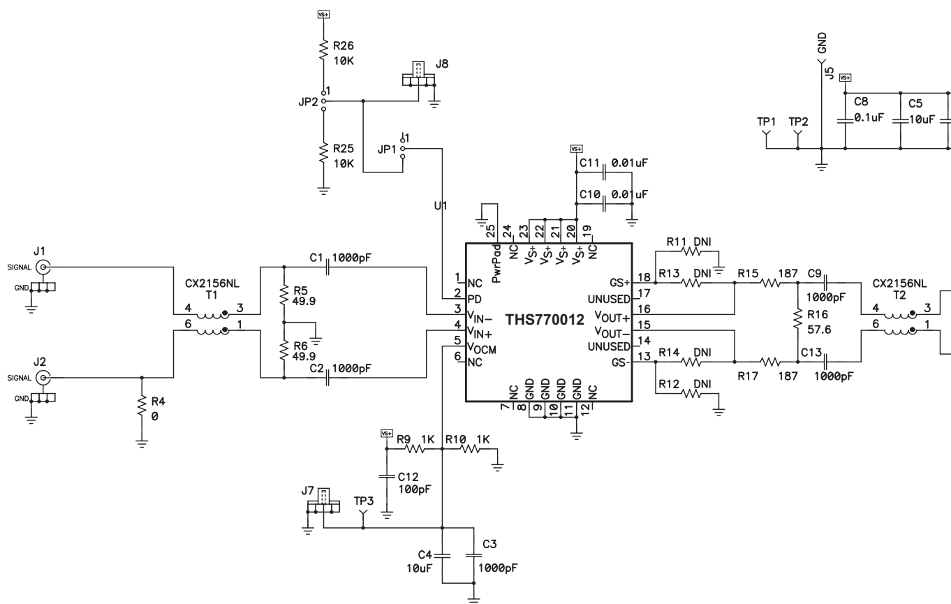
Figure 34. THS770012IRGE EVM Schematic
