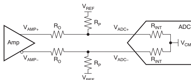
Figure 38. Resistor Network to DC Level Shift Common-Mode Voltage
