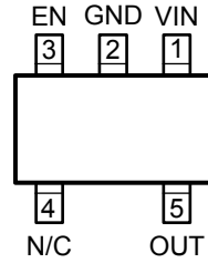
MIC5306-x.xBD5
