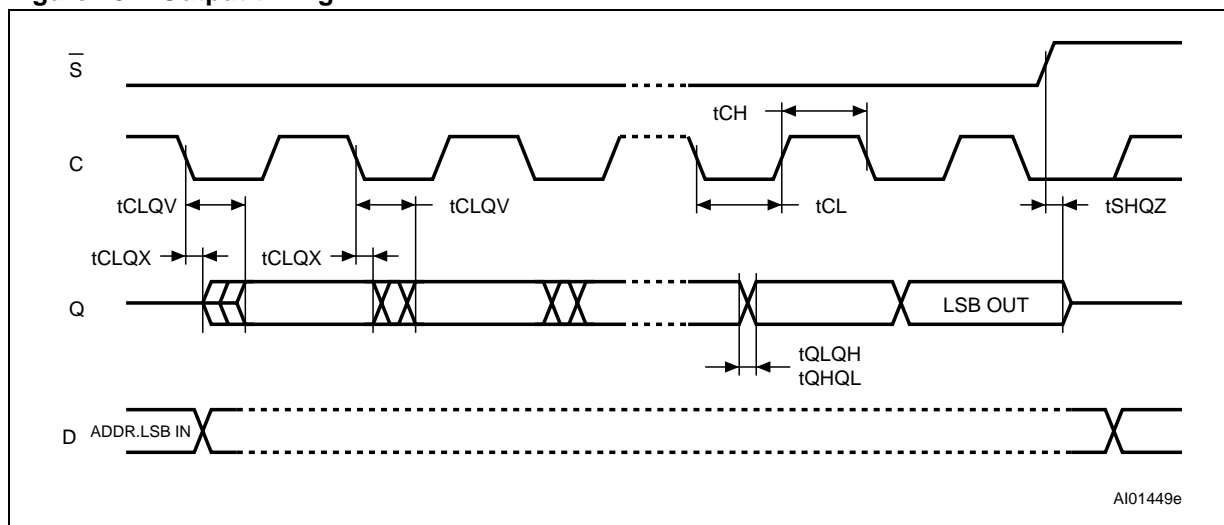
Figure 28. Output timing
