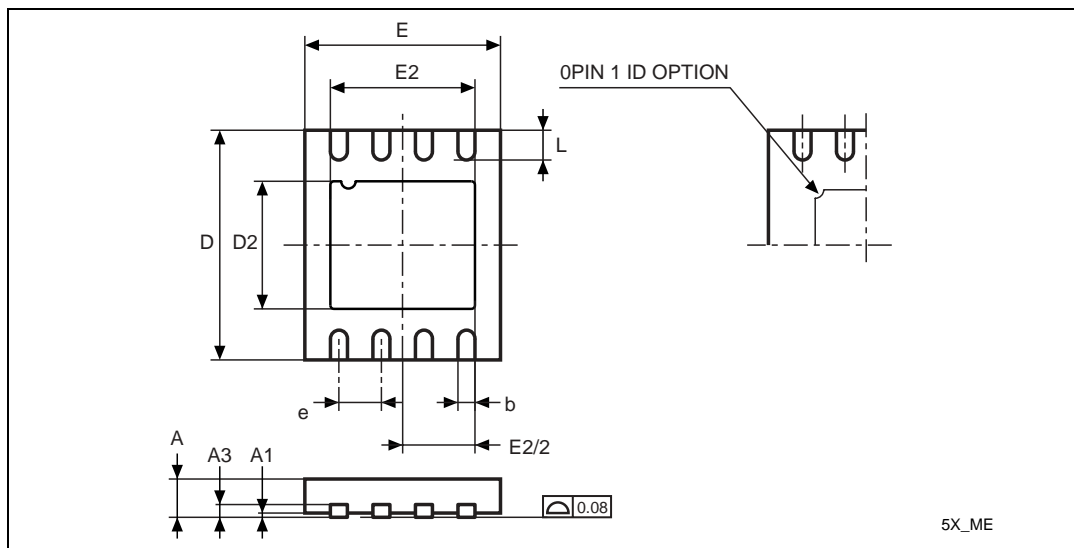
Figure 31. QFN8L (MLP8) 8-lead, quad flat package no lead, 6 × 5 mm, package outline
