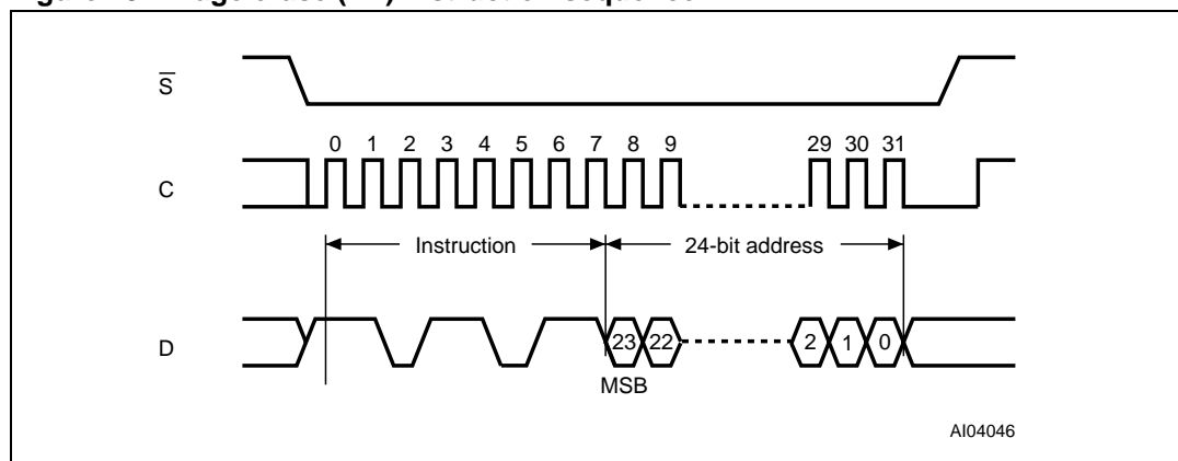
Figure 18. Page erase (PE) instruction sequence
