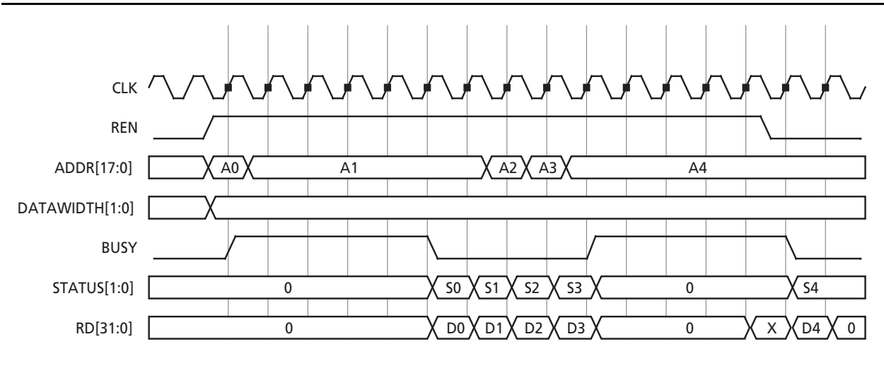
Figure 2-38 • Read Waveform (Pipe Mode, 32-bit access)
