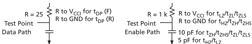
Figure 2-115 • AC Loading
