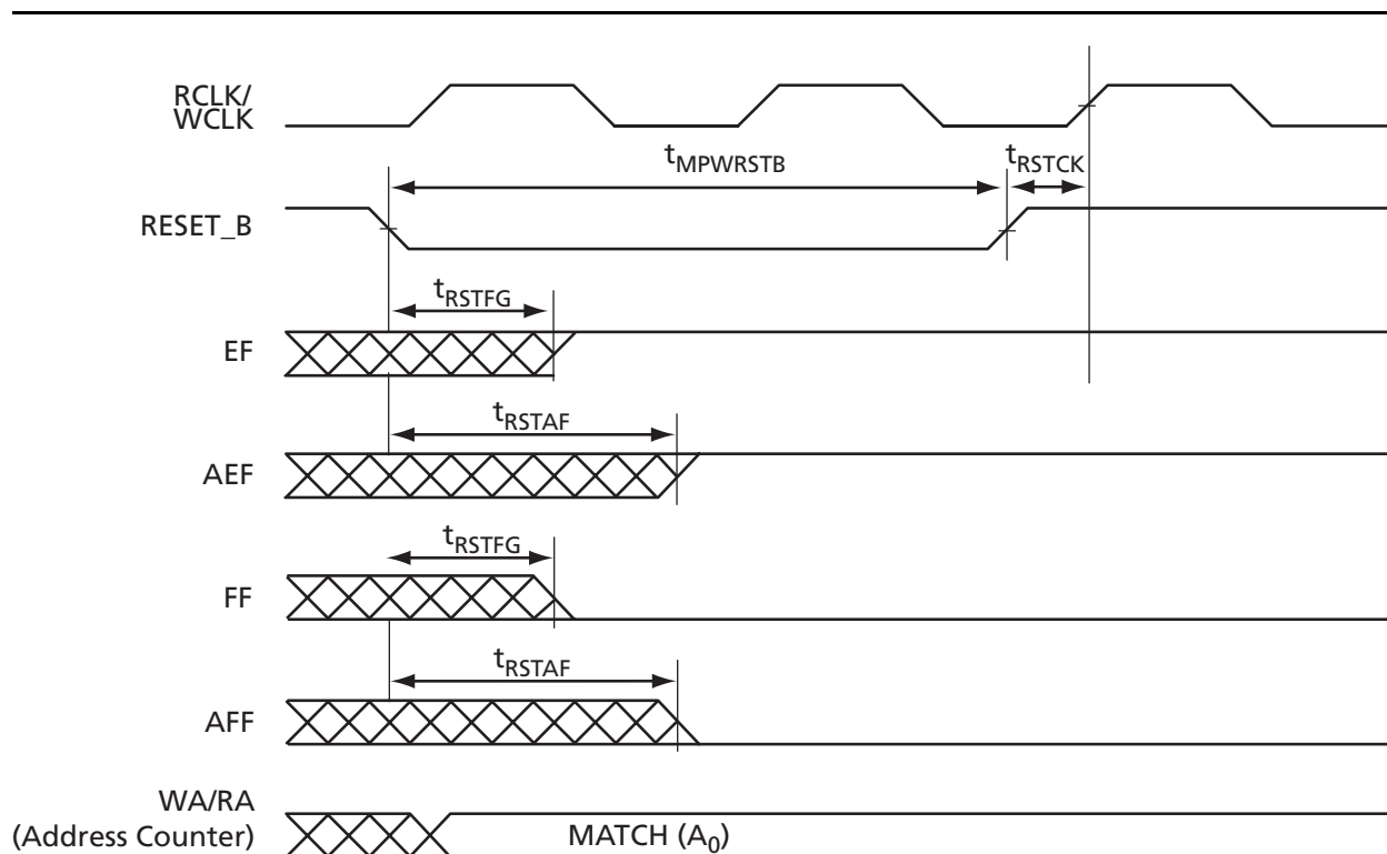
Figure 2-59 • FIFO Reset
