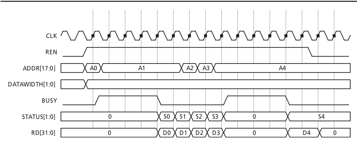
Figure 2-37 • Read Waveform (Non-Pipe Mode, 32-bit access)
