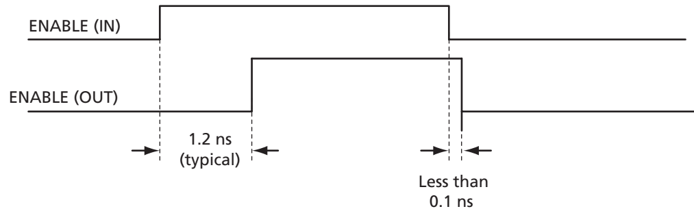
Figure 2-101 • Timing Diagram (option 2: enables skew circuit)
