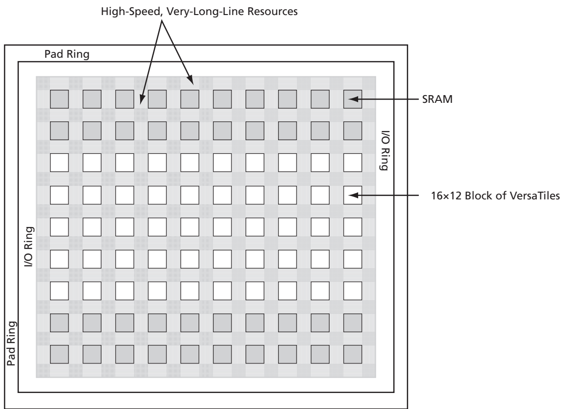
Figure 2-10 • Very-Long-Line Resources
