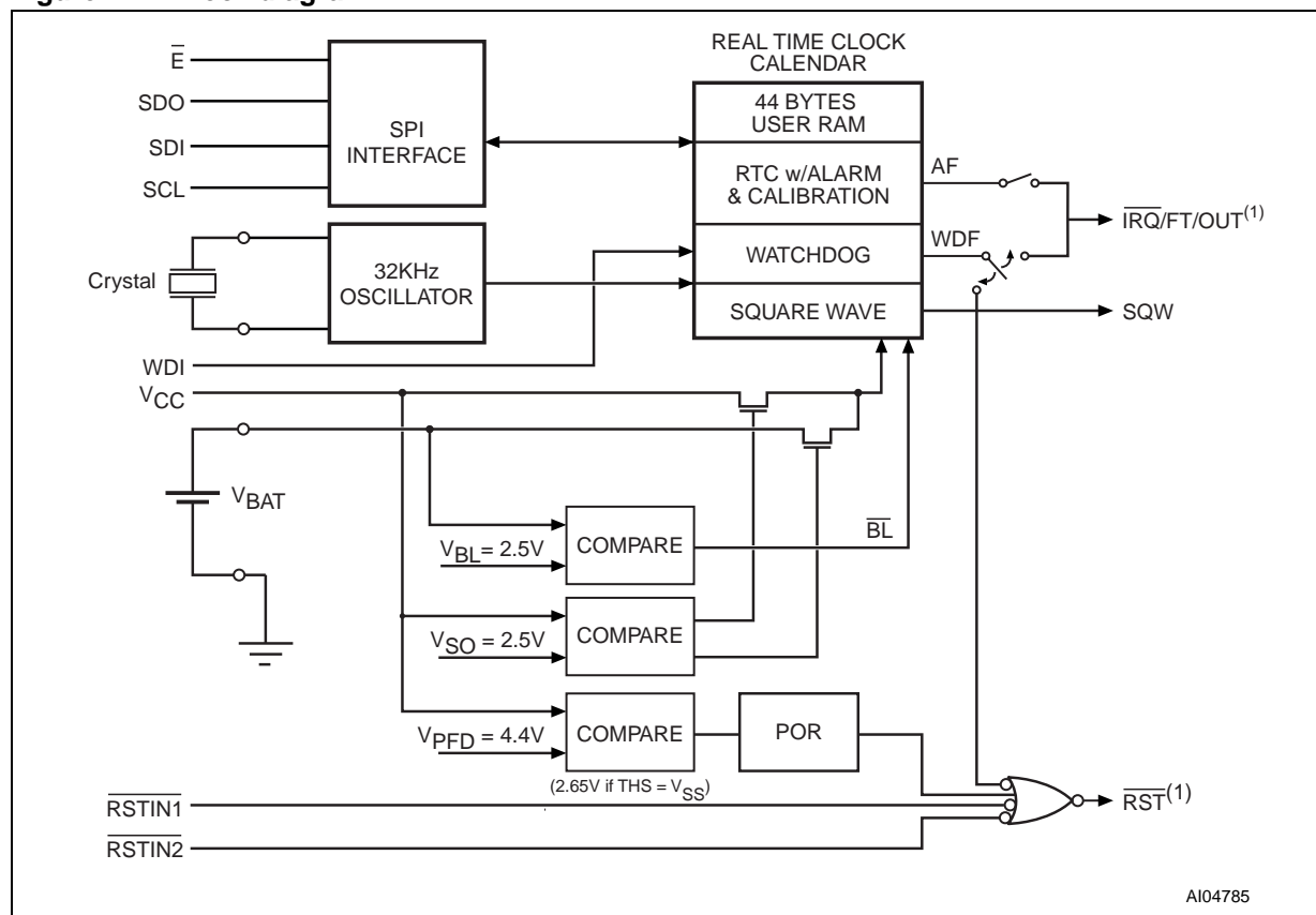
Figure 4. Block diagram
