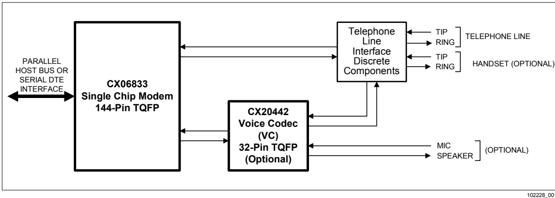
Figure 1-1. SMXXD Modem Simplified Interface Diagram
