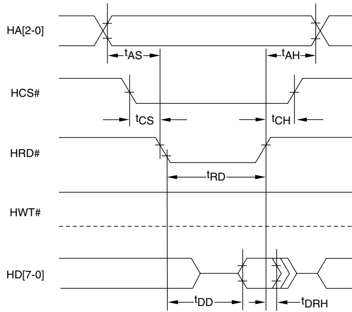
Figure 3-8. Waveforms - Parallel Host Bus
