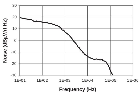
AAT3200 Noise Spectrum
