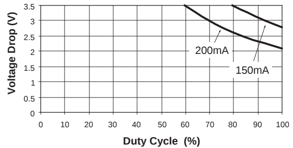
Device Duty Cycle vs. V_{DROP} ( V_{OUT} = 2.5V @ 25^\circ C )
