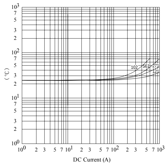
@ DC Current VS. Temp. Rise Curve
