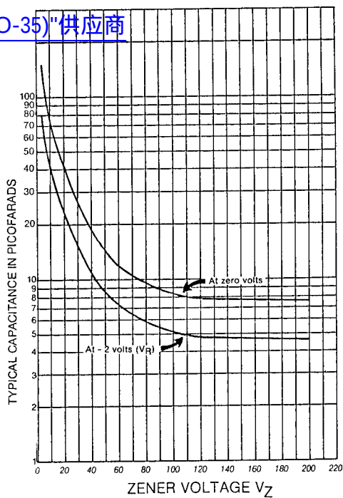
FIGURE 4 CAPACITANCE VS. ZENER VOLTAGE (TYPICAL)
