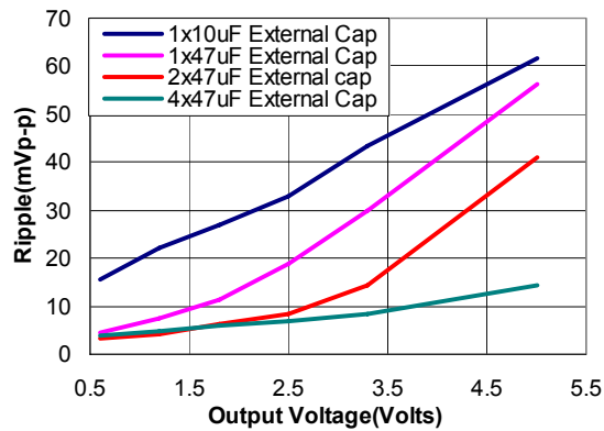
Figure 41. Output ripple voltage for various output voltages with external 1x10 µF, 1x47 µF, 2x47 µF or 4x47 µF ceramic capacitors at the output (12A load). Input voltage is 12V.
