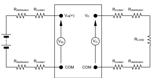
Figure 38. Output Ripple and Noise Test Setup.
