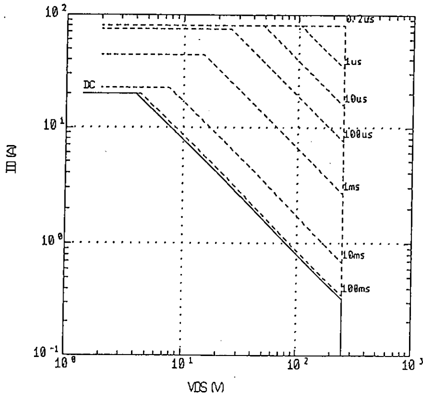
Safe operating area ID=f(VDS): D=0.01, Tc=25^{\circ}C
