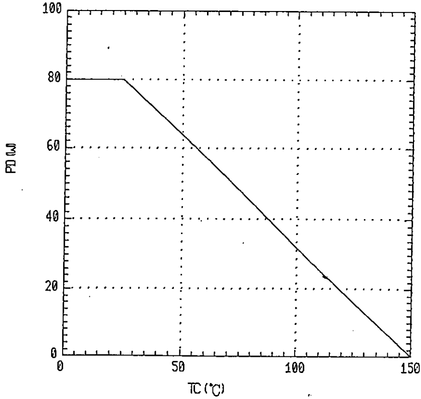
Power Dissipation PD=f(TC)
