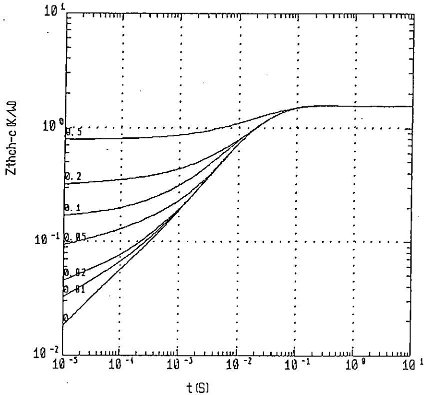
Transient thermal impedance Z_{thch-c}=f(t) parameter: D=t/T
