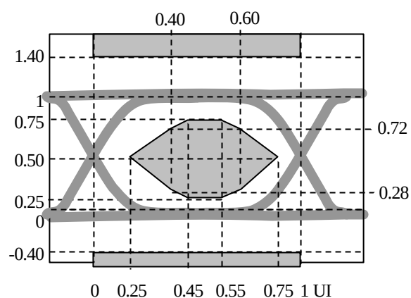
Fig. 6.1.2 MASK for IEEE802.3ae
