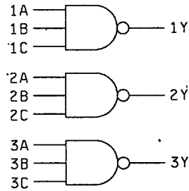
FIGURE 3. Logic diagram.
