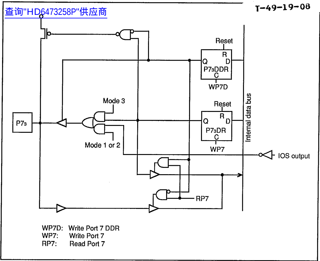
Figure 5-16. Port 7 Schematic Diagram (Pin P73)
