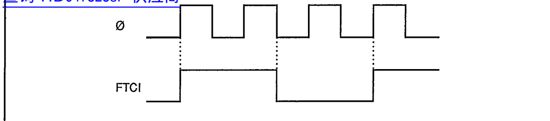
Figure 7-6. Minimum External Clock Pulse Width
