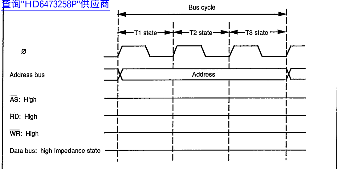
Figure 3-16. Pin States during On-Chip Register Field Access Cycle
