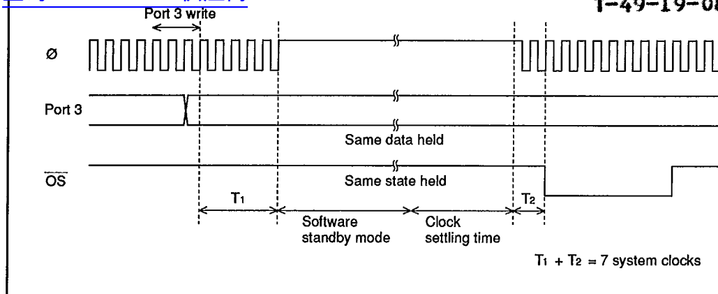
Figure 6-5. Output Strobe Timing in Software Standby Mode
