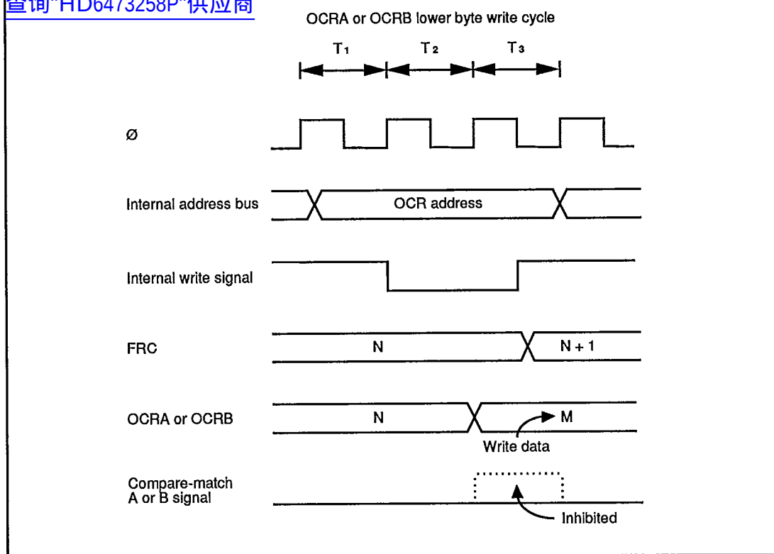
Figure 7-19. Contention between OCR Write and Compare-Match
