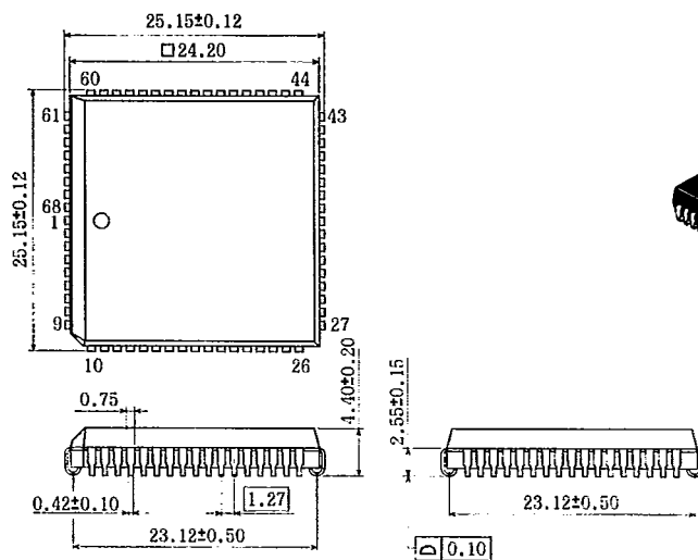
Figure E-4. Package Dimensions (CP-68)
