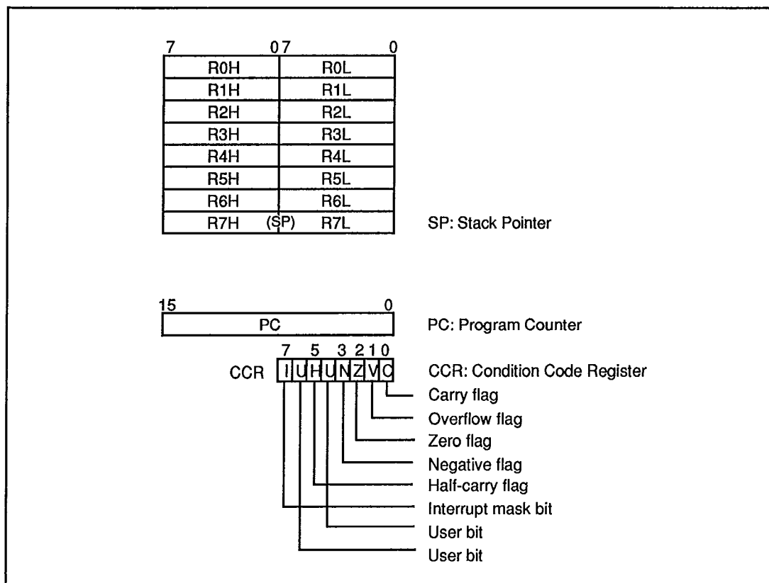
Figure 3-1. CPU Registers
