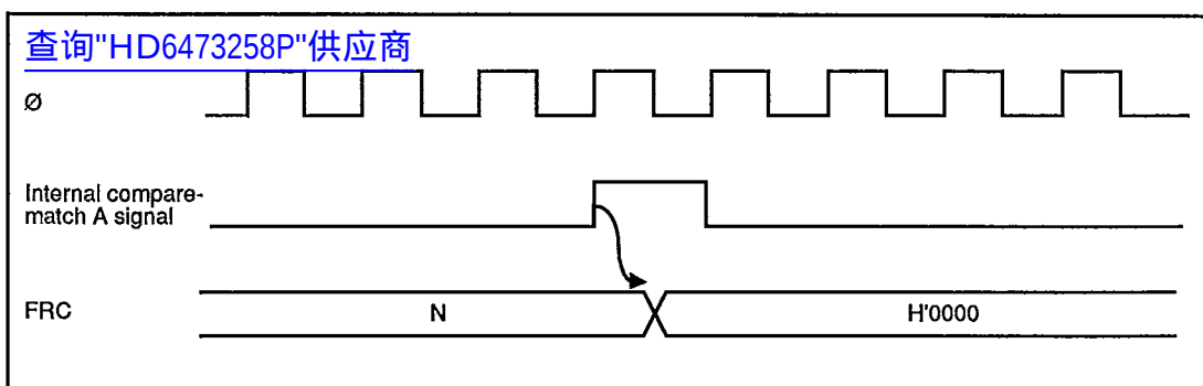
Figure 7-8. Clearing of FRC by Compare-Match A
