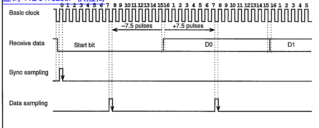
Figure 9-5. Sampling Timing (Asynchronous Mode)
