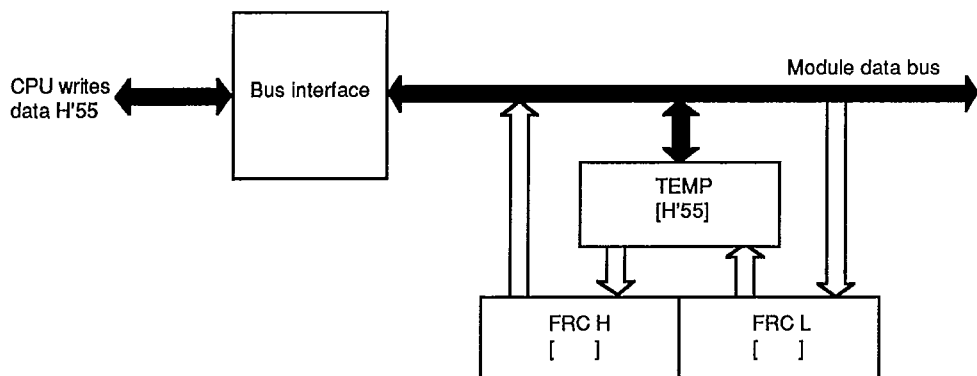
Figure 7-3 (b). Read Access to FRC (When FRC Contains H'AA55)
