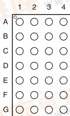
YFF PACKAGE (TOP VIEW)
