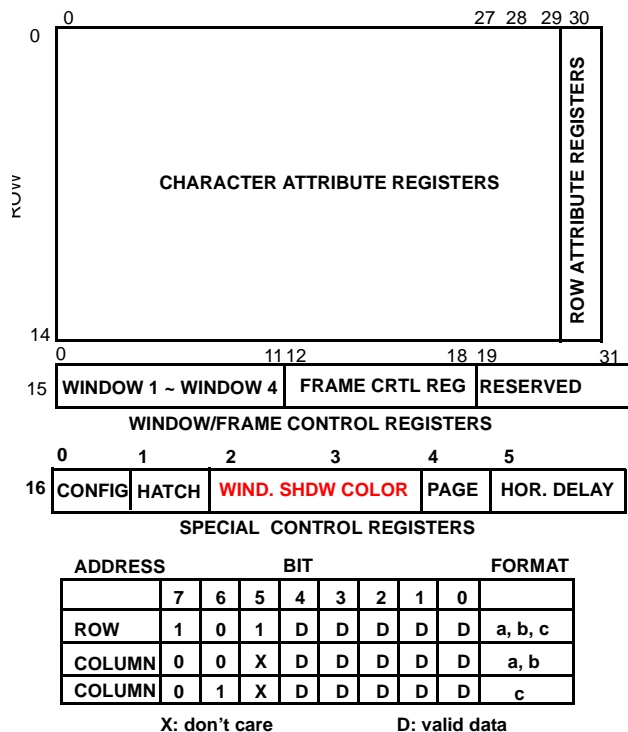
Figure 8. Address Bit Patterns for Attribute/Control Data
