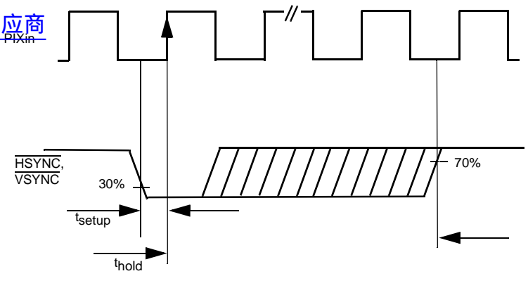
Figure 3. Setup/Hold Timing Diagram
