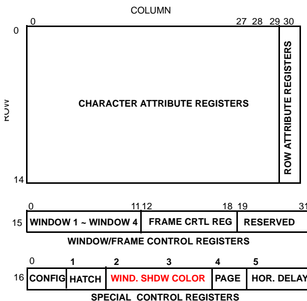
Figure 10. Memory Map of Attribute/Control Registers
