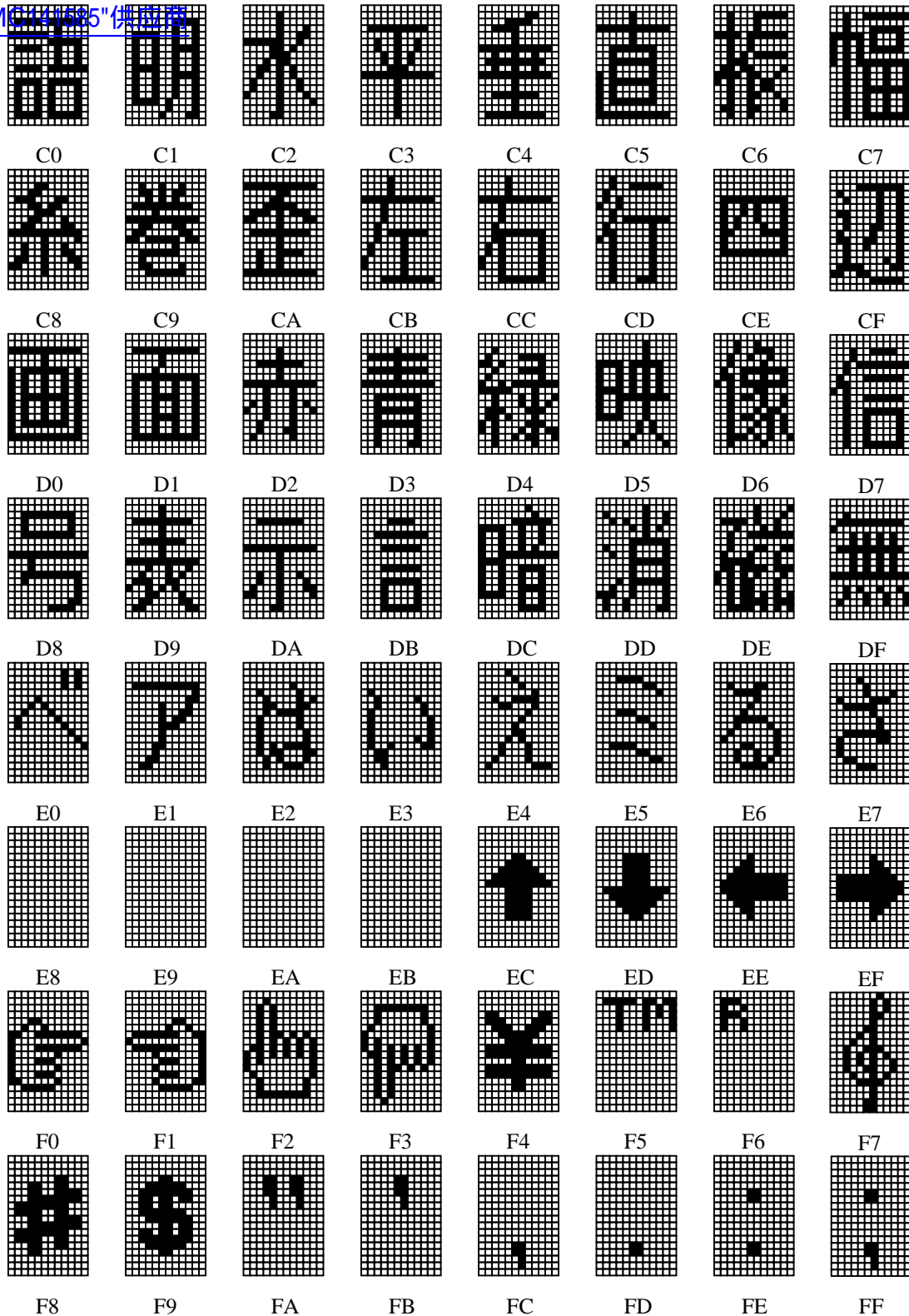
Figure 6. ROM contents for PAGE 4
