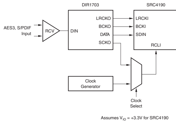
Figure 9. Interfacing the SRC4190 to the DIR1703 Digital Audio Interface Receiver
