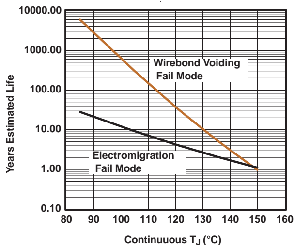
Operating Life Derating Chart
