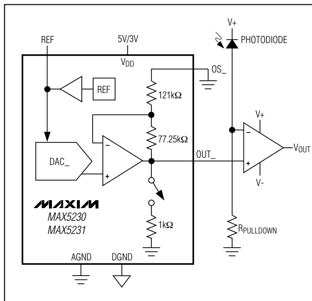
Figure 8. Digital Calibration
