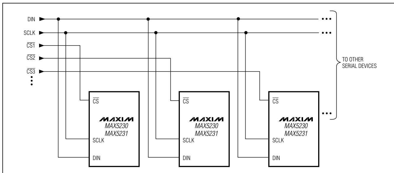
Figure 9. Multiple MAX5230/MAX5231s Sharing a Common DIN Line
