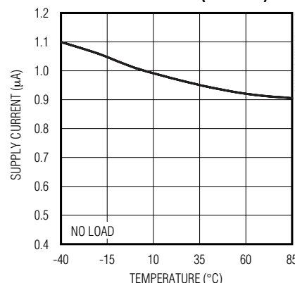
FULL POWER-DOWN SUPPLY CURRENT vs. TEMPERATURE (MAX5231)
