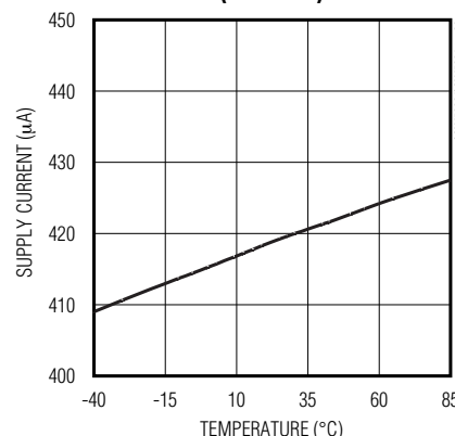
FULL POWER-DOWN SUPPLY CURRENT vs. TEMPERATURE (MAX5230)
