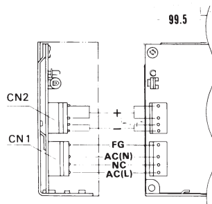
“-J” Option Molex Connectors
