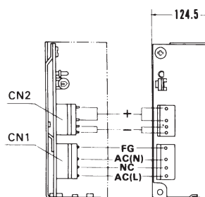
“-J” Option Molex Connectors
