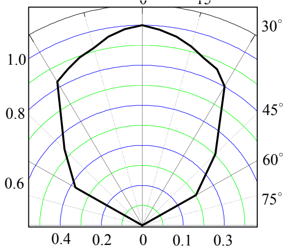
RELATIVE TRANSMISSION
