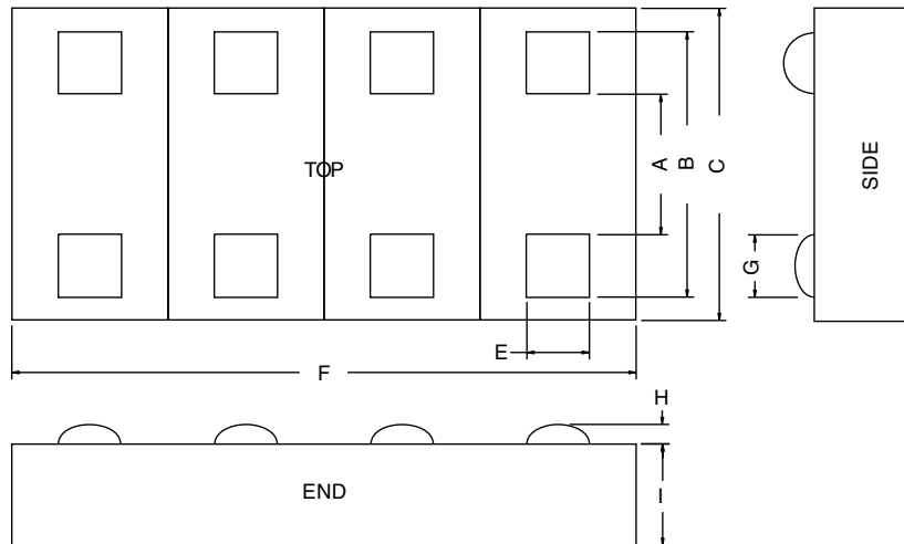
PACKAGE OUTLINE
