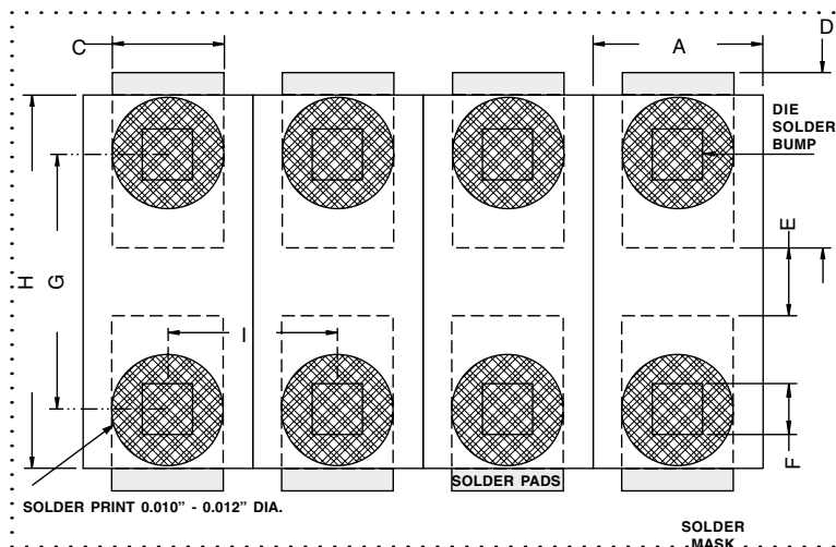
MOUNTING PAD LAYOUT - Option 1
