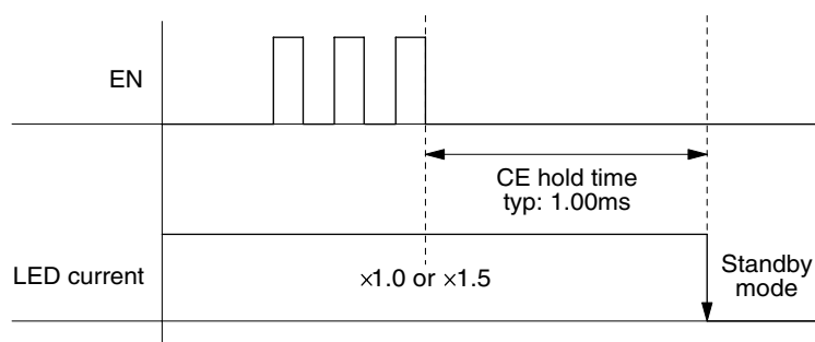
EN input signal and internal enable signal "CE"
