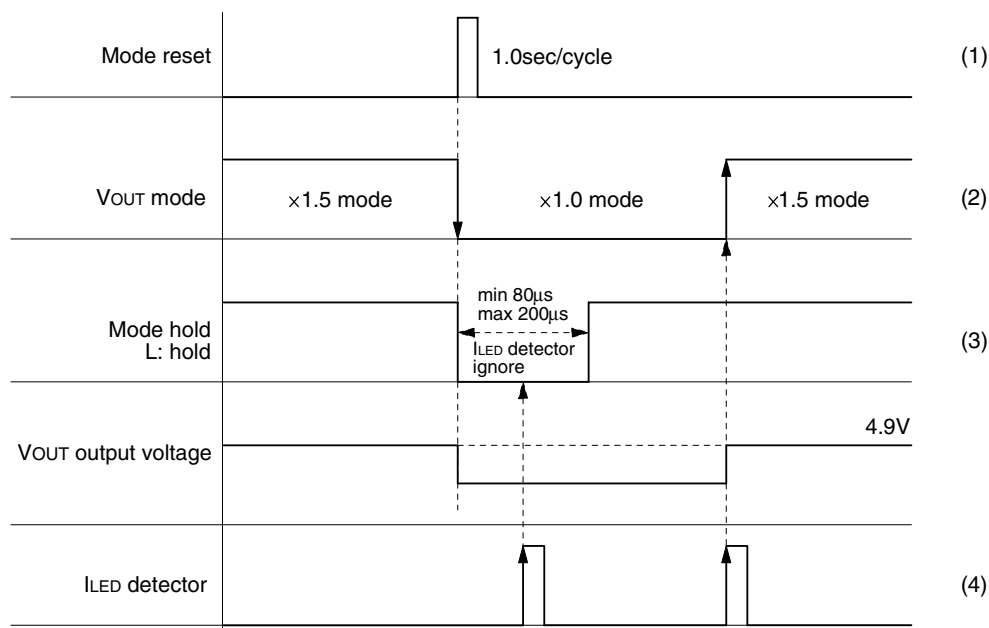
Switching from ×1.5 mode to ×1.0 mode due to mode reset signal
