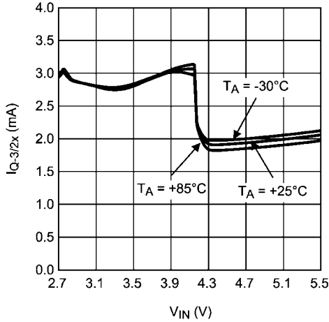
Quiescent Current vs Input Voltage 查询"LM3535"供应商
