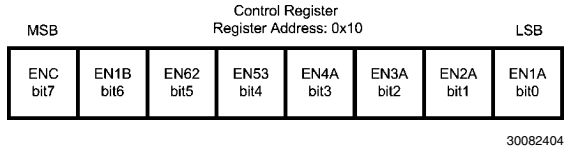
FIGURE 4. Diode Enable Register Description Internal Hex Address: 0x10
