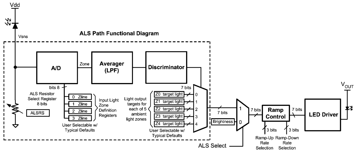
FIGURE 14. Ambient Light Sensor Functional Block Diagram
