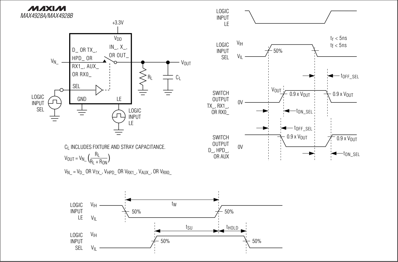
Figure 1. Switching Time
