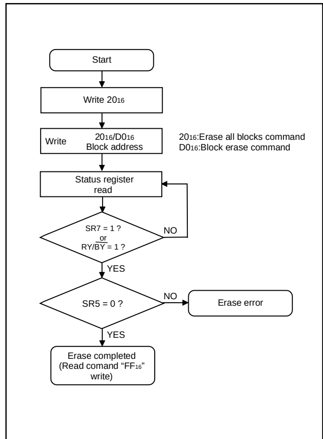
Fig. 61 Erase flowchart
