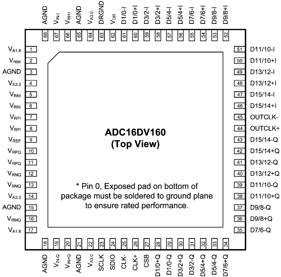
Pin-Out of ADC16DV160
