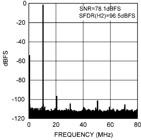
Spectral Response @ 10.1 MHz
