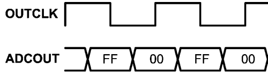
FIGURE 18. Fixed Pattern at ADC Output with Default SPI Register Values
