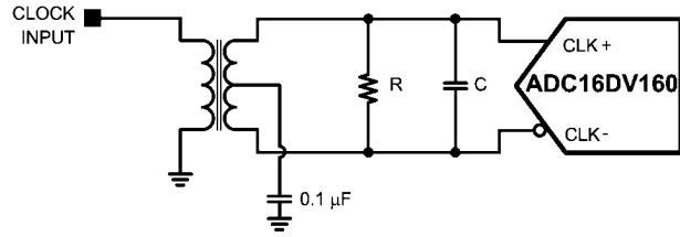
FIGURE 10. Differential Clocking, Transformer Coupled
