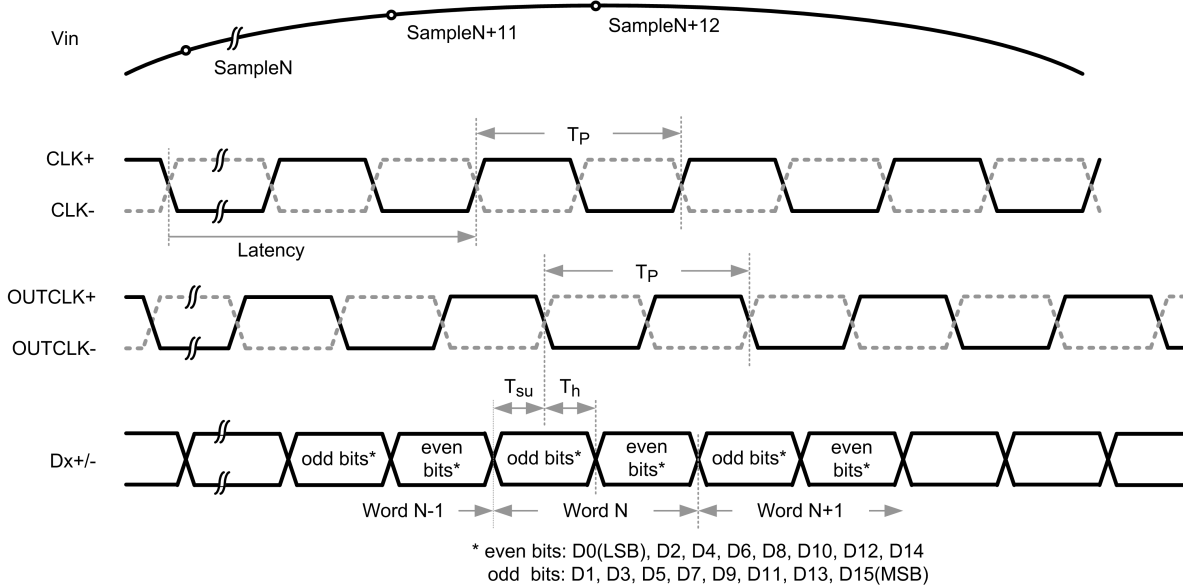
FIGURE 1. Digital Output Timing
