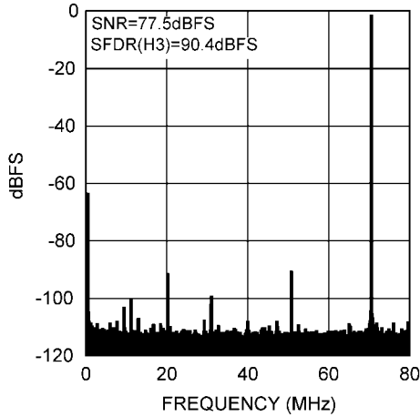
Spectral Response at 70 MHz
