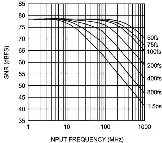
FIGURE 12. SNR with given Jitter vs. Input Frequency
