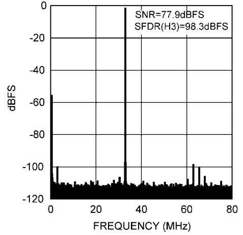
Spectral Response @ 32.5 MHz
