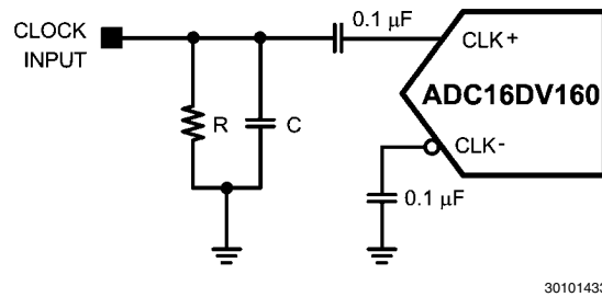
FIGURE 11. Singled-Ended 1.8V Clocking, Capacitive AC Coupled
