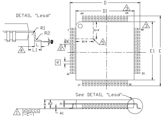
Figure 9.1 64 Pin TQFP Package Outline, 10X10X1.4 Body, 12x12 mm Footprint
