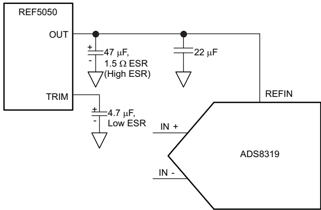
Figure 60. Direct External Reference Driving Circuit
