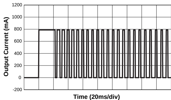
Over-Current Protection
