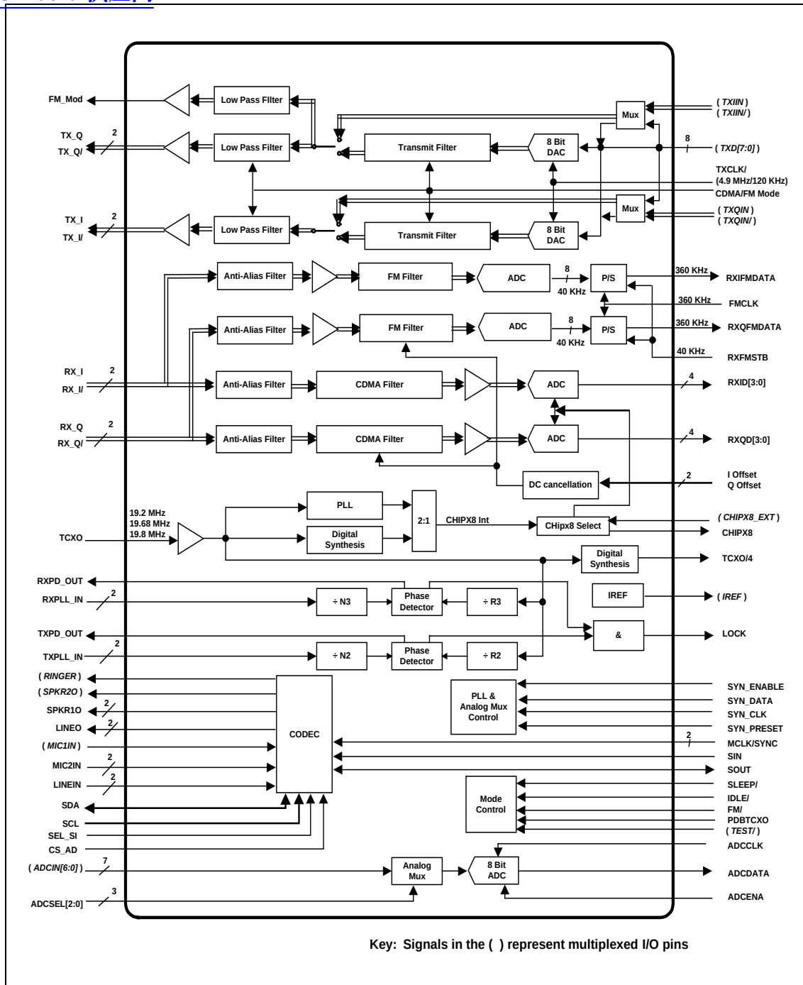
Figure 4. CX20470 System Block Diagram (100-Pin \mu BGA Package)
