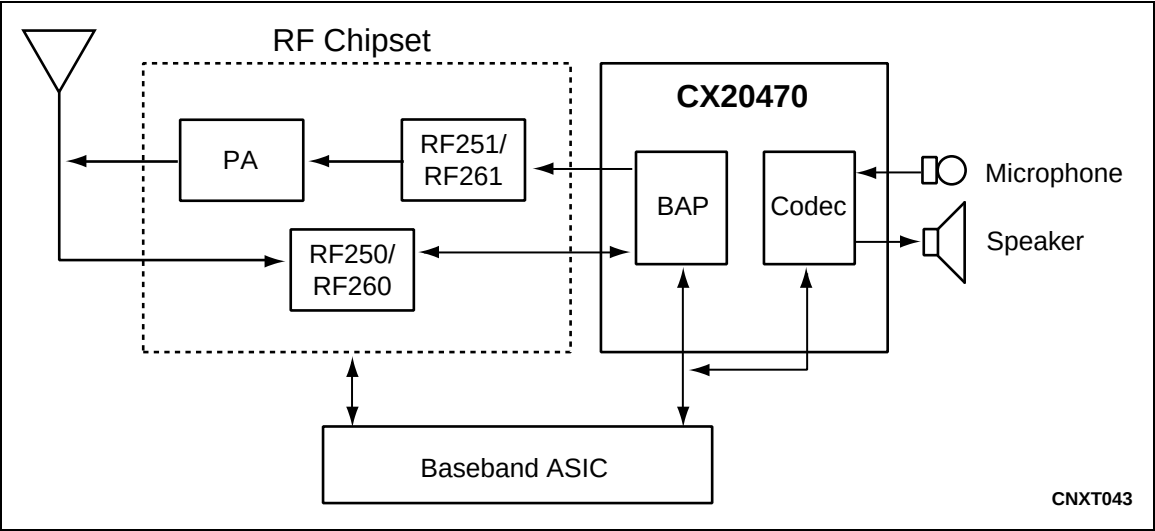
Figure 3. CX20470 General Block Diagram
