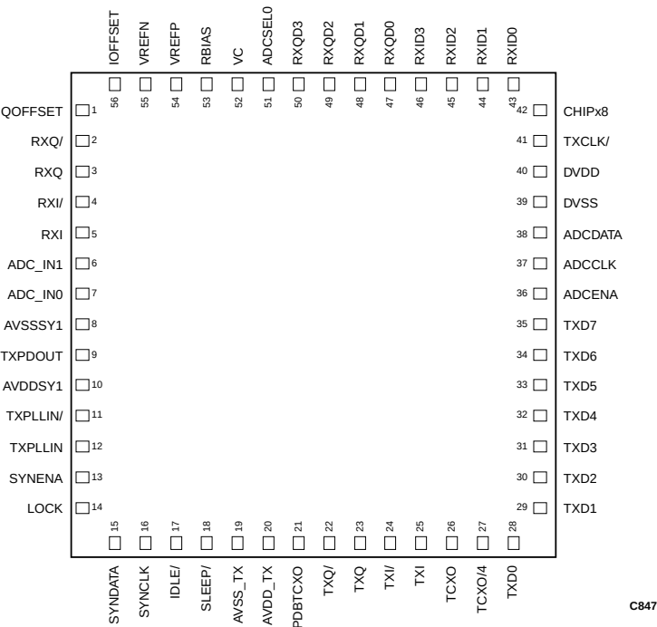
Figure 2. CX20470 BAP Pinout – 56-Pin LGA Package
