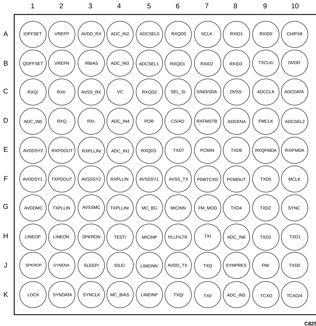
Figure 1. CX20470 BAP Pinout – 100-Pin \mu BGA Package
