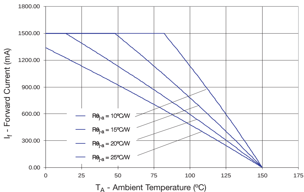
Figure 14: Maximum forward current vs. ambient temperature, based on T JMAX = 150°C.
