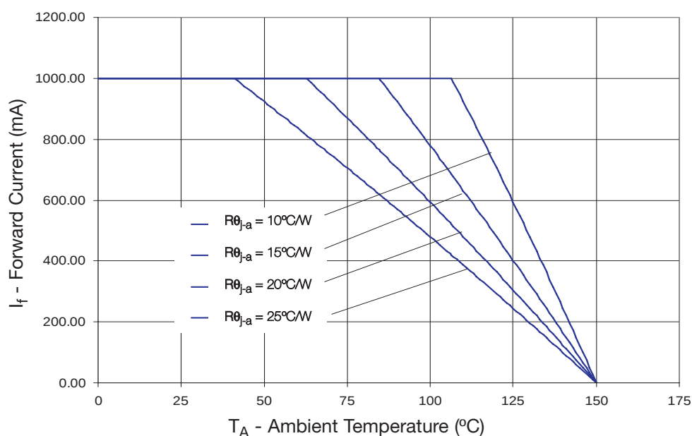
Figure 15: Maximum forward current vs. ambient temperature, based on T JMAX = 150°C.
