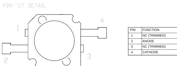
Figure 8. 2-Lead Gullwing Pin Out Diagram.
