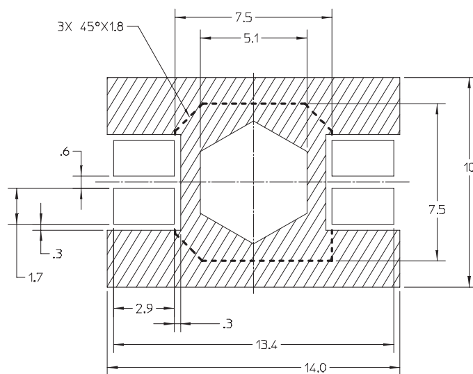
Figure 3. 4-Lead Gullwing Package Solder Pad Layout.
