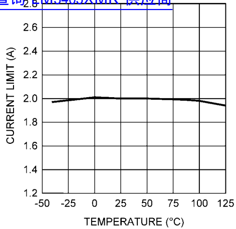
Current Limit vs Temperature 查询"LM3405XMK"供应商
