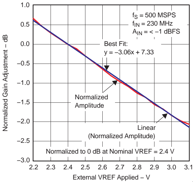
Figure 53. ADS5463 Signal Gain Adjustment versus External VREF
