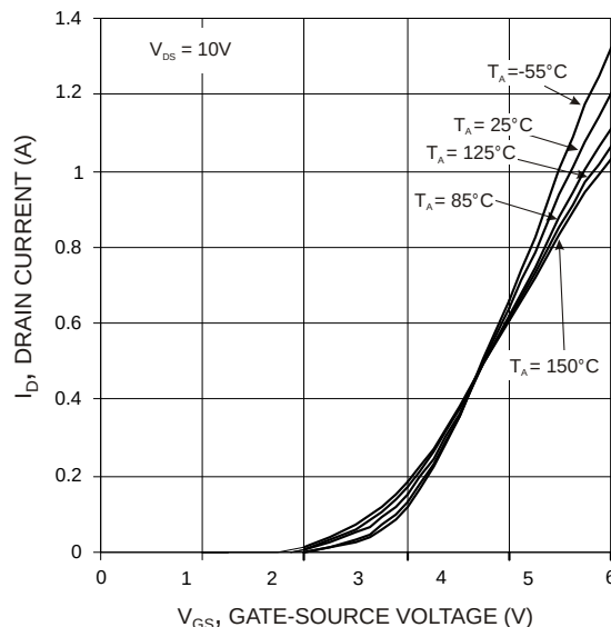
Fig. 11 Transfer Characteristics
