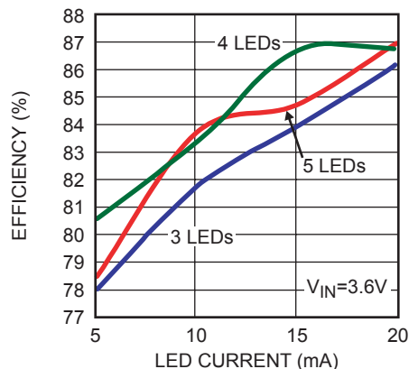
Efficiency vs LED Current
