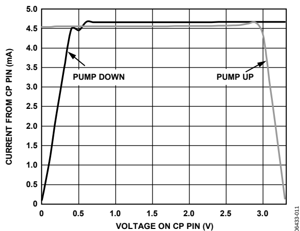
Figure 7. Charge Pump Characteristics @ V_{CP} = 3.3\text{ V}
