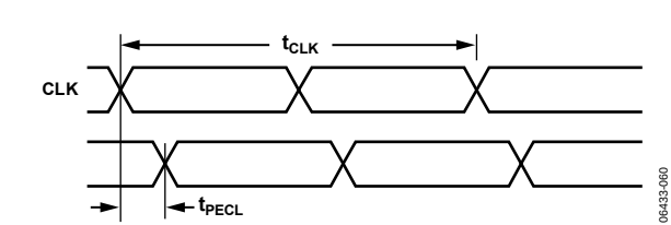
Figure 2. CLK/ \overline{CLK} to Clock Output Timing, DIV = 1
