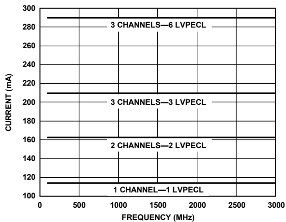
Figure 5. Current vs. Frequency, Direct-to-Output, LVPECL Outputs
