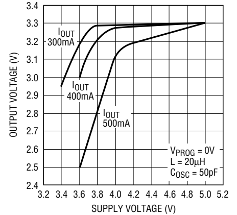
Dropout Characteristics at Different Load Currents ( V_{\text{OUT}} = 3.3\text{V} )
