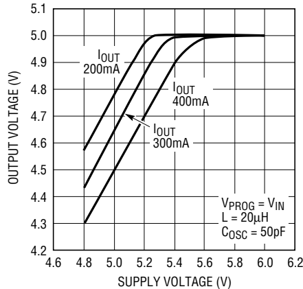
Dropout Characteristics at Different Load Currents ( V_{\text{OUT}} = 5\text{V} )
