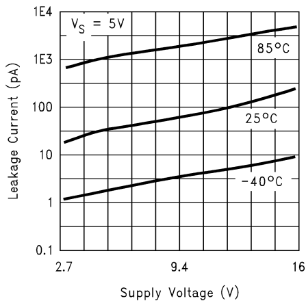
Leakage Current vs. Supply Voltage
