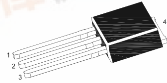
1.Base 2.Collector 3.Emitter 4.Collector TO-251 Plastic Package
