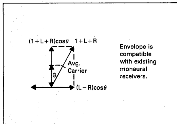
FIGURE 3 — MOTOROLA C-QUAM®
