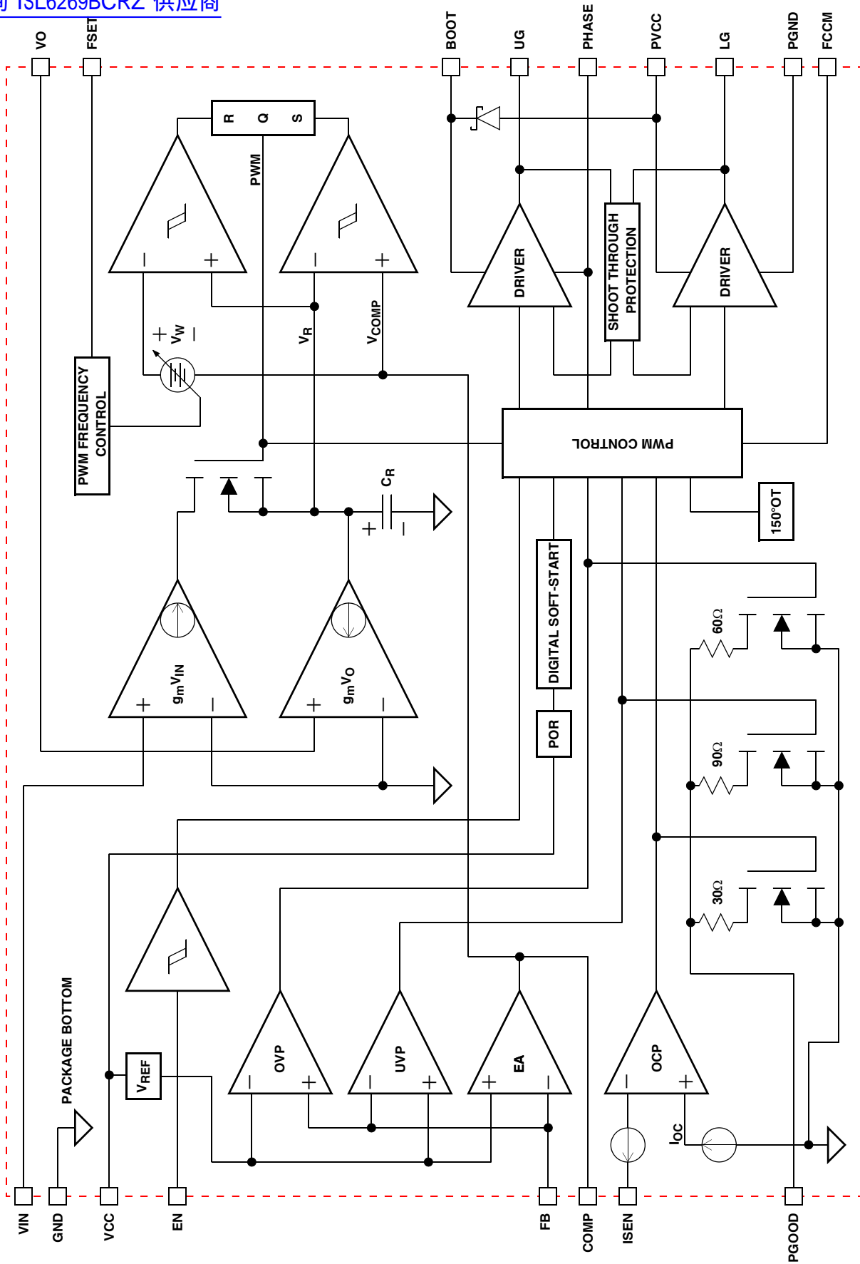
FIGURE 1. SCHEMATIC BLOCK DIAGRAM
