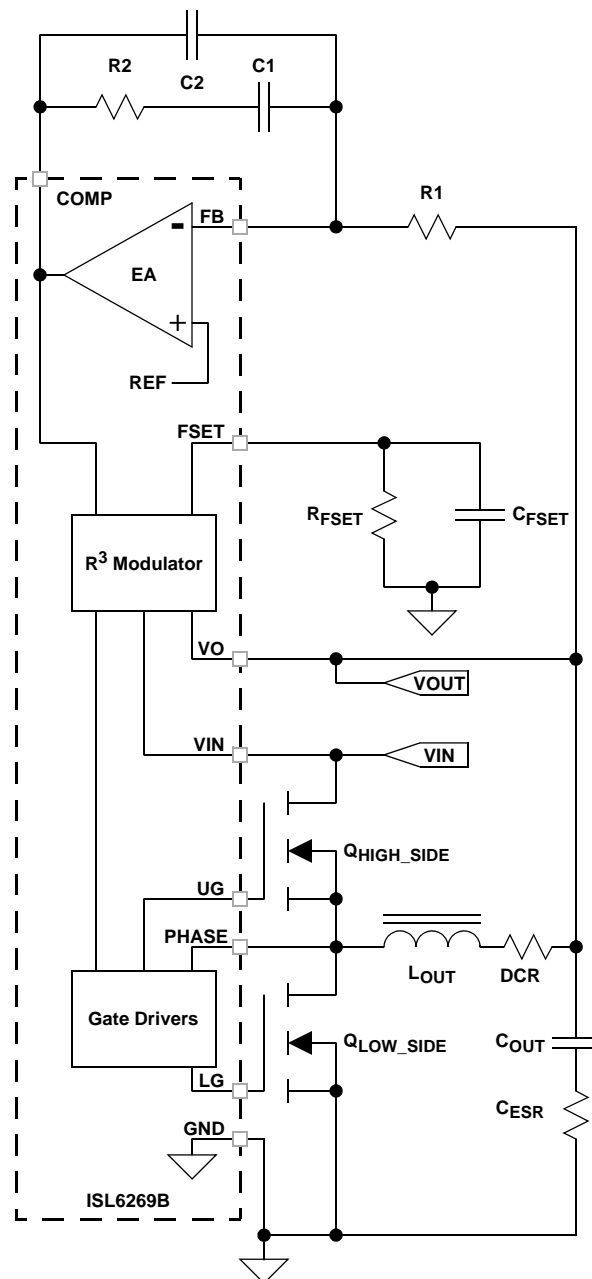
Your local Intersil representative can provide a PC-based tool that can be used to calculate compensation network component values and help simulate the loop frequency response. The compensation network consists of the internal error amplifier of the ISL6269B and the external components R1, R2, C1, and C2 as well as the frequency setting components R_{FSET} and C_{FSET} , are identified in the schematic Figure 5.
