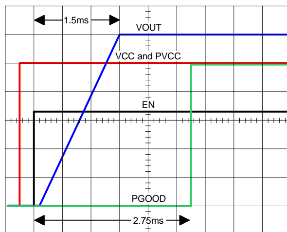
FIGURE 3. SOFT-START SEQUENCE
