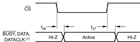
Figure 10. Enable and Disable Timing for Digital Outputs
