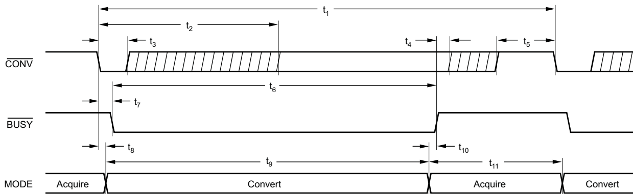
Figure 3. Basic Conversion Timing
