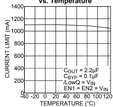
DC/DC Current Limit vs. Temperature
