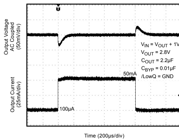
LDO2 Load Transient LowQ Mode
