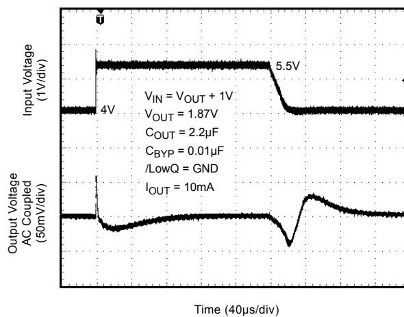
LDO2 Line Transient LowQ Mode
