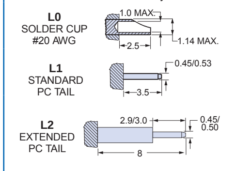
Detail A Terminal Styles
