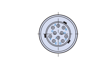
VG96934D10*L0 10 pin in-line unshrouded receptacle with two piece shielded aluminum backshell. 6 mm cable entry. Black zinc plating. Not for new design. Replaced by Style K. Maximum weight 15 grams.
