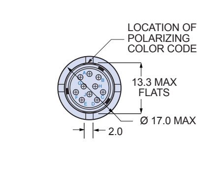
VG96934D10*L0 10 pin in-line unshrouded receptacle with two piece shielded aluminum backshell. 6 mm cable entry. Black zinc plating. Not for new design. Replaced by Style K. Maximum weight 15 grams.
