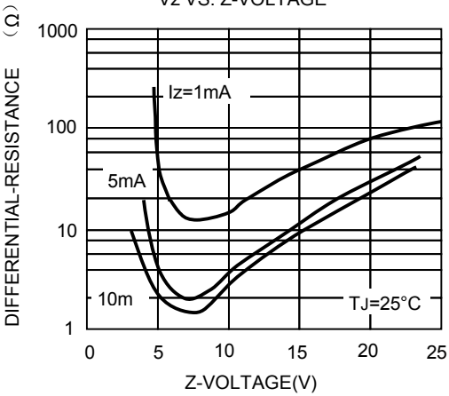
FIG.10 - DIFFERENTIAL Z-RESISTANCE Vz VS. Z-VOLTAGE
