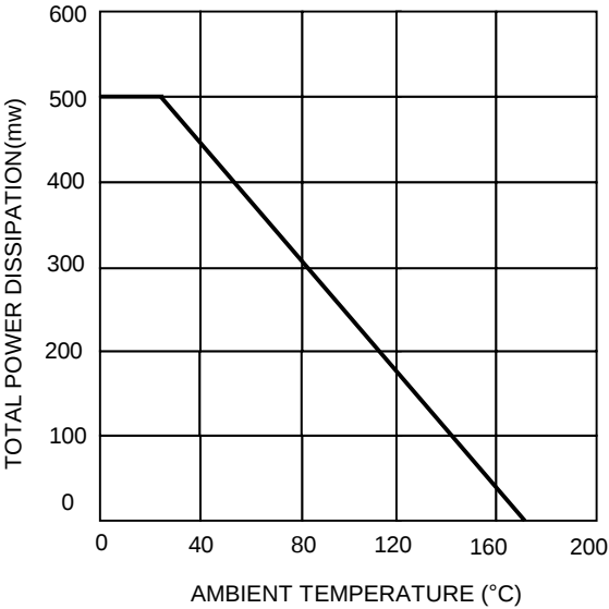
FIG. 2 - TOTAL POWER DISSIPATION VS. AMBIENT TEMPERATURE
